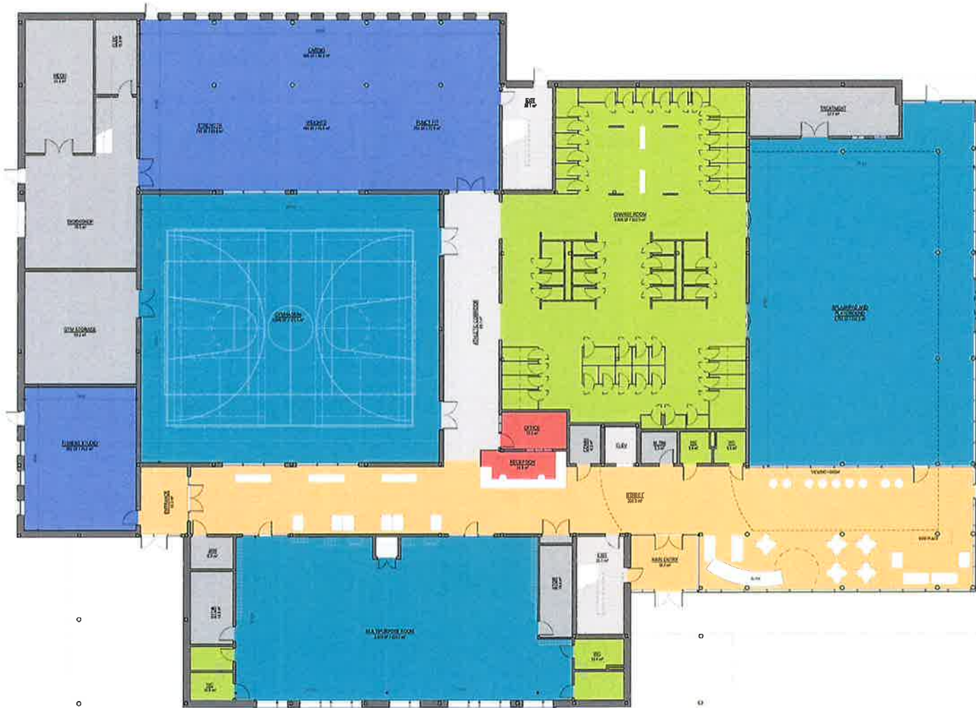
YMCA MONCTON NORTH - LEVEL 1 FLOORPLAN 1:100
